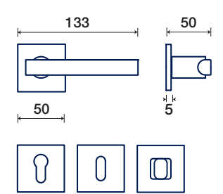
rosette - bocchette 5 mm rosettes - escutcheon
